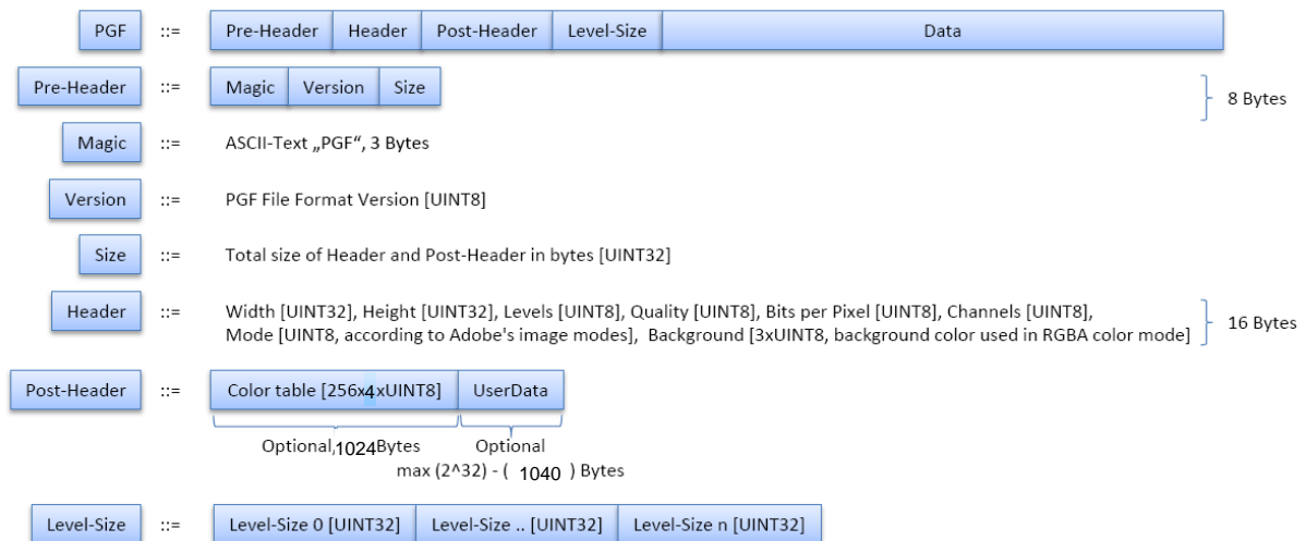
Figure 1: PGF header structure
